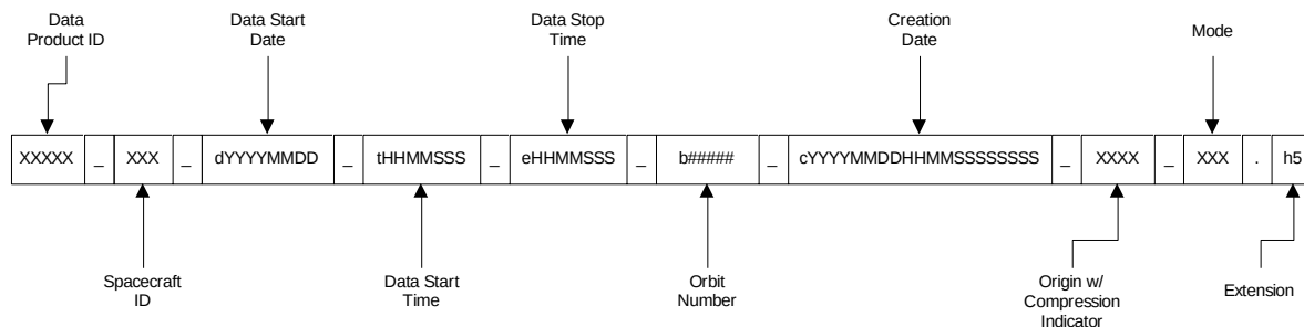
Figure 3.4.1-1. S-NPP/JPSS Data Products File-Naming Convention
