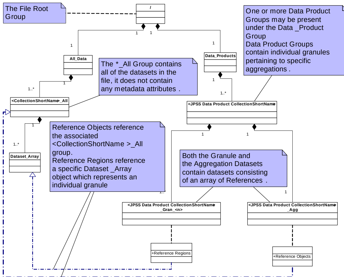
Figure 3.5.2.1-2. JPSS HDF5 UML Diagram (For RDRs only)
