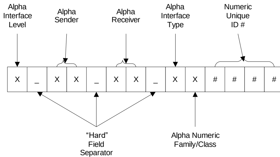
Figure 3.1-1. JPSS Interface and Service Mnemonic Definition
