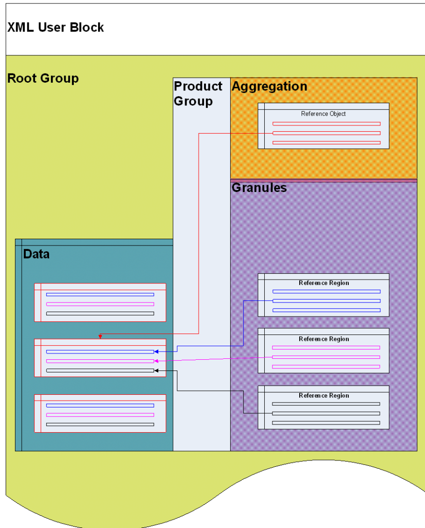
Figure 3.5-1. JPSS HDF5 Conceptual Diagram
