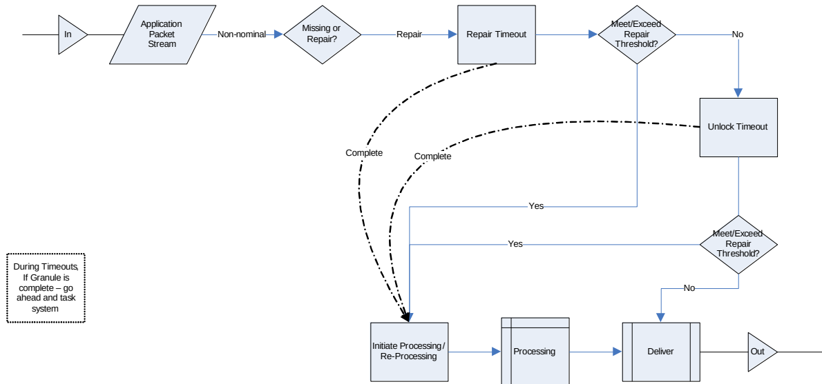
Figure 3.5.8.4.2-1, Non-Nominal Repaired RDR Granule Data Flow Diagram, provides a graphical depiction of the data flow for Repaired RDR granules
