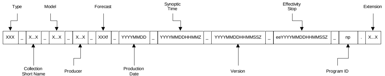
Figure 3.4.5-1, Ancillary File-Naming Convention
