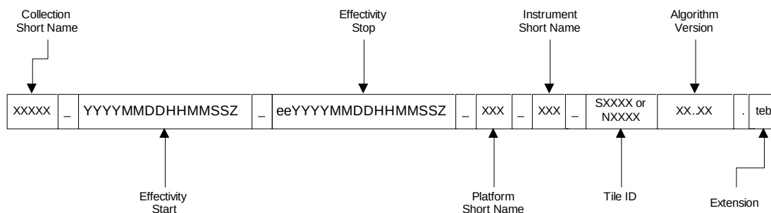
Figure 3.4.5.1-1, IDPS Terrain Database File-Naming Convention
