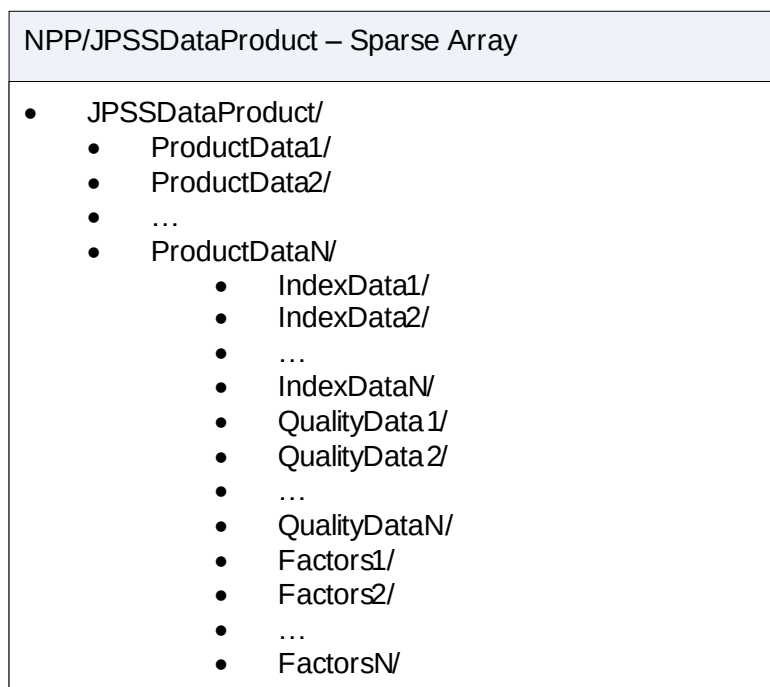
Figure 3.5.4.3.1-1, JPSS Sparse Array Style General Profile Example
