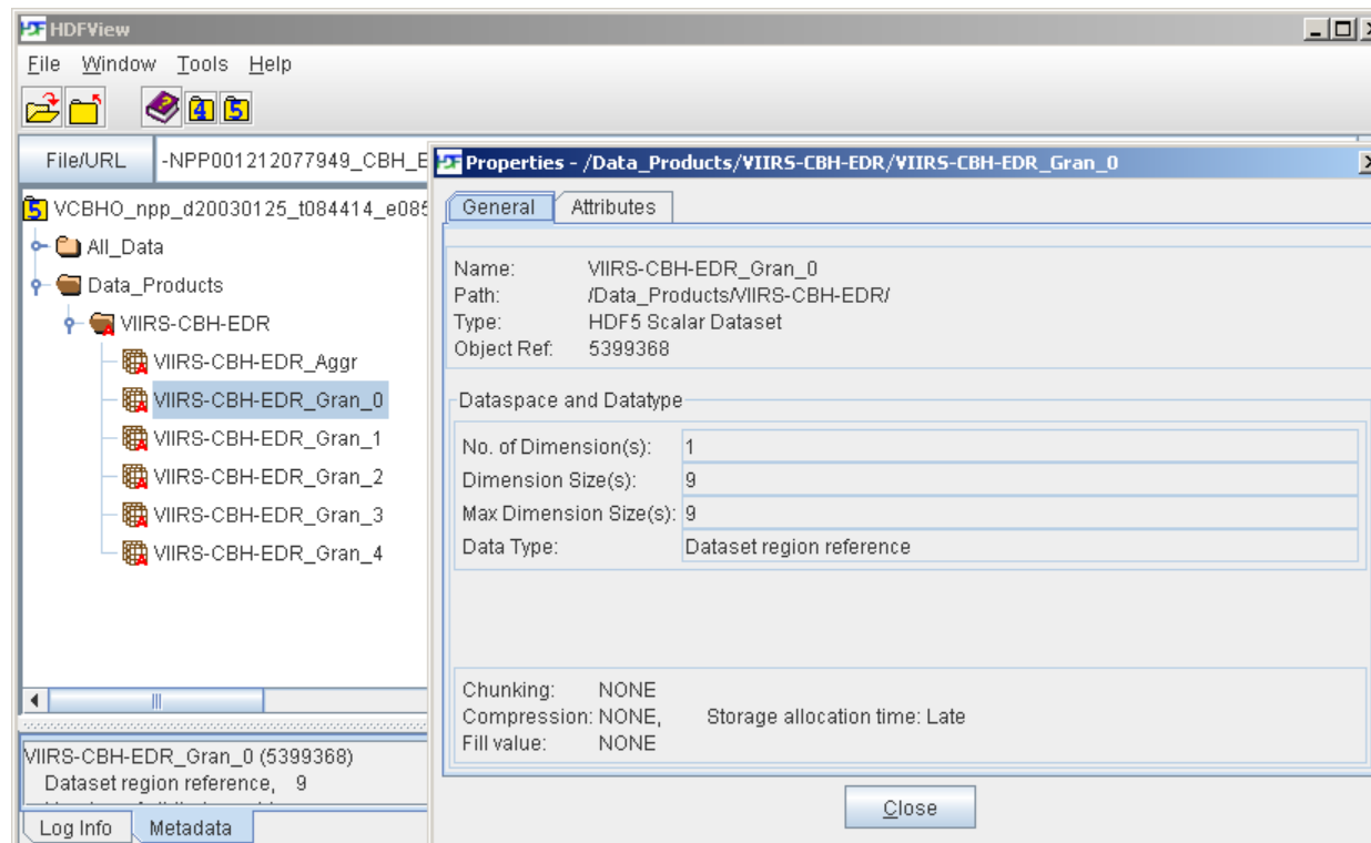
Figure 3.5.3-1, VIIRS CBH EDR Granule Properties Example
