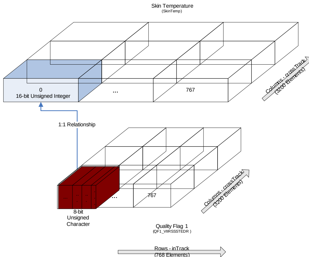
Figure 3.5.5-1, 2-Dimensional Quality Flag Example – SST
