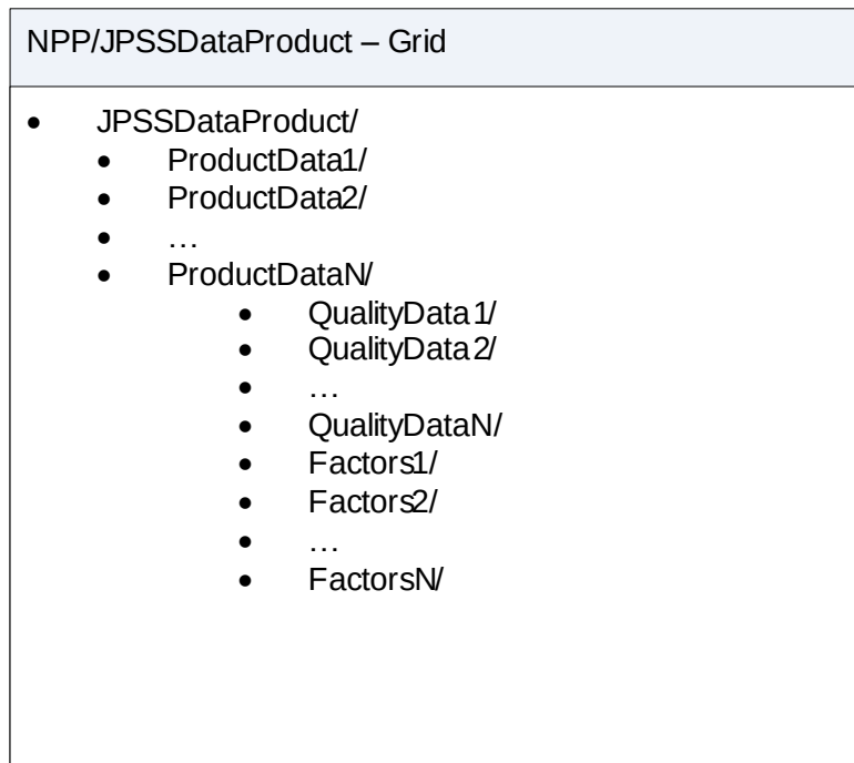
Figure 3.5.4.2.1-1, JPSS Grid Style General Profile Example
