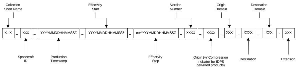
Figure 3.4.4-1, Auxiliary File-Naming Convention
