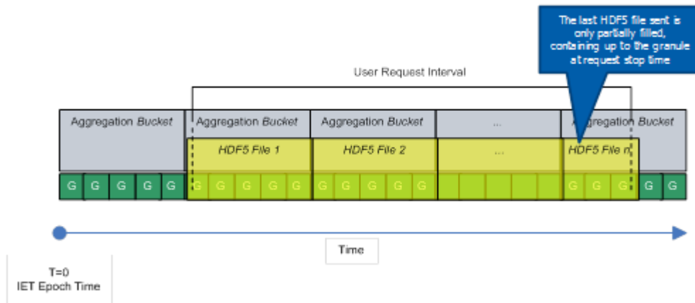
Figure 3.5.12-2, Aggregation User Request Example 1
