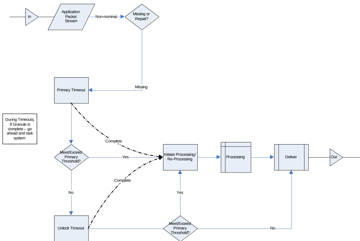
Figure 3.5.8.4.1-1, Non-Nominal Missing/Late RDR Granule Data Flow Diagram
