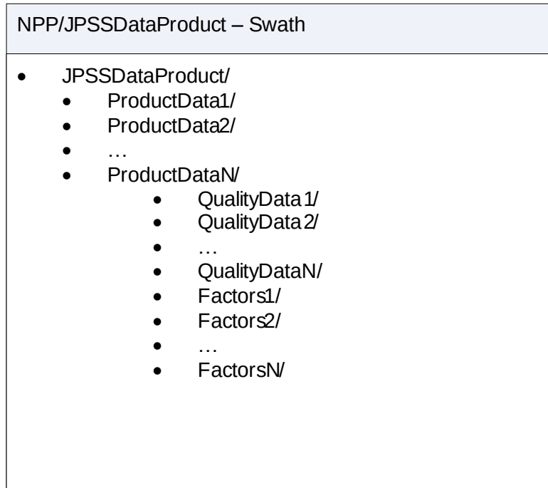
Figure 3.5.4.1.1-1, JPSS Swath Style General Profile Example
