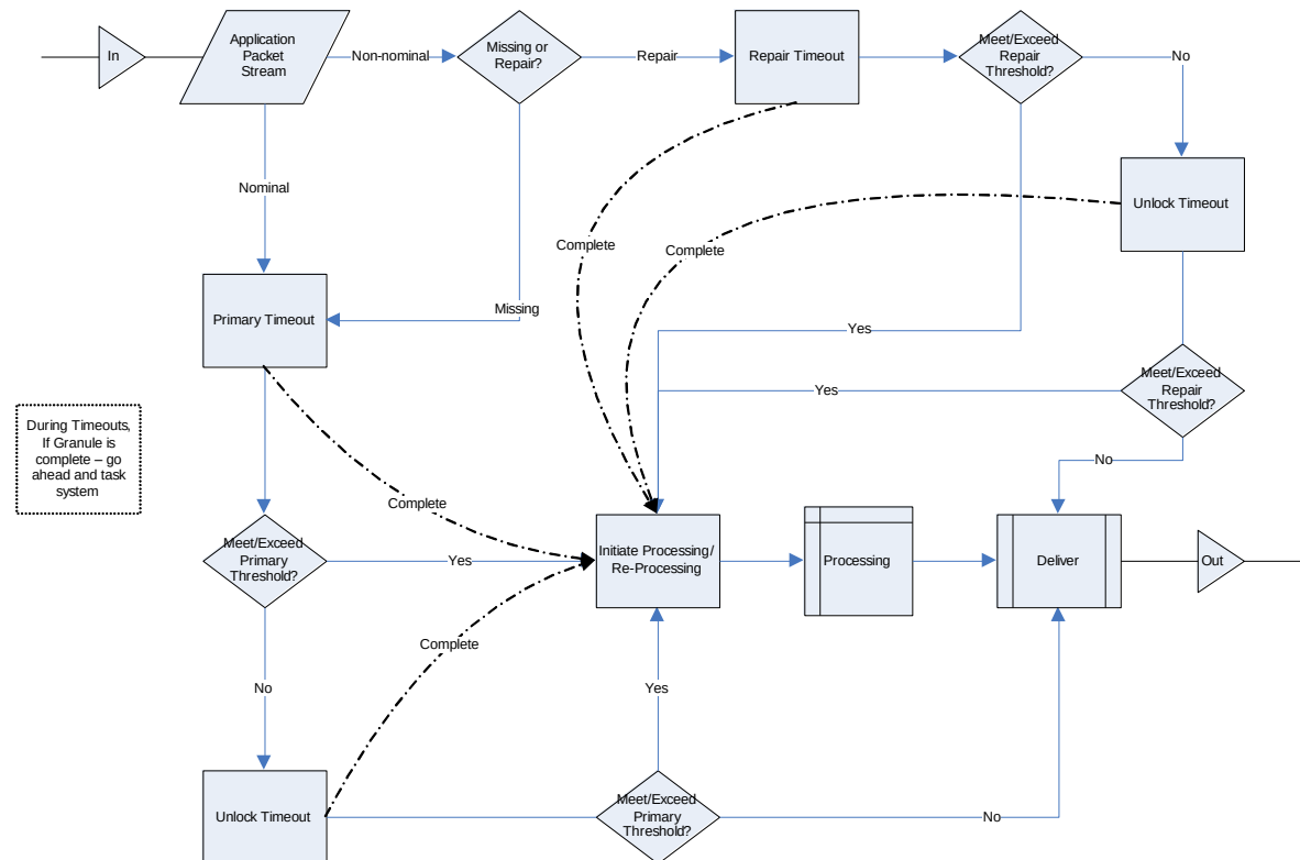
Figure 3.5.8.1-1, RDR Granule Data Flow Diagram
