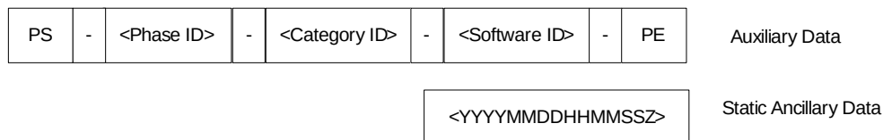
Figure 3.4.4-2, Provenance Version Identifier Convention
