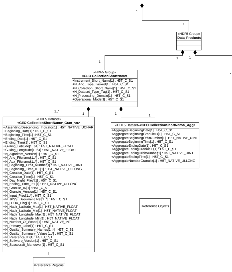
Figure 3.5.7.1-2, Generalized Geolocation HDF5 Diagram – Packaging On
