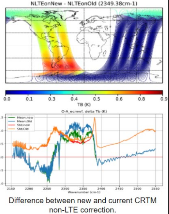
Figure 2. TMP 18-05 made noteworthy progress in handling non-local thermodynamic equilibrium (NLTE) emission, improving NWP model assimilation of hyperspectral SWIR radiance observations.
