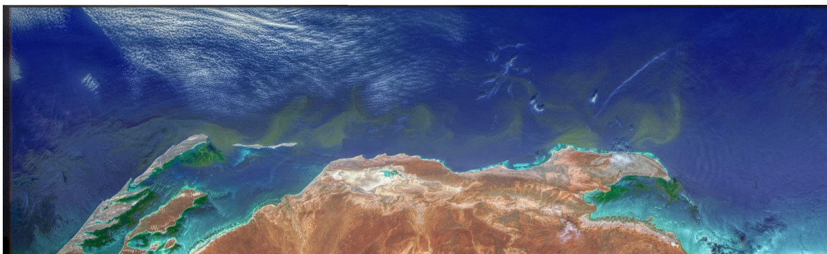
Figure 11. SeaHawk acquired its first fully stable image over northwestern Australia, showing the impressive capability of the SeaHawk instrument when it is operating on a stable platform.
