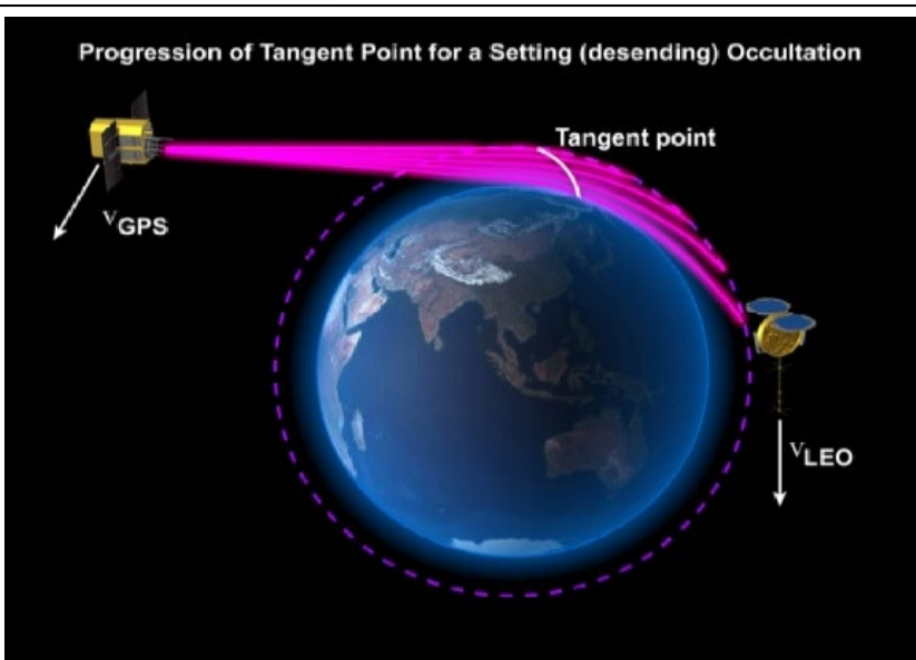
Figure 19. Bistatic radio occultation remote sensing geometry.
