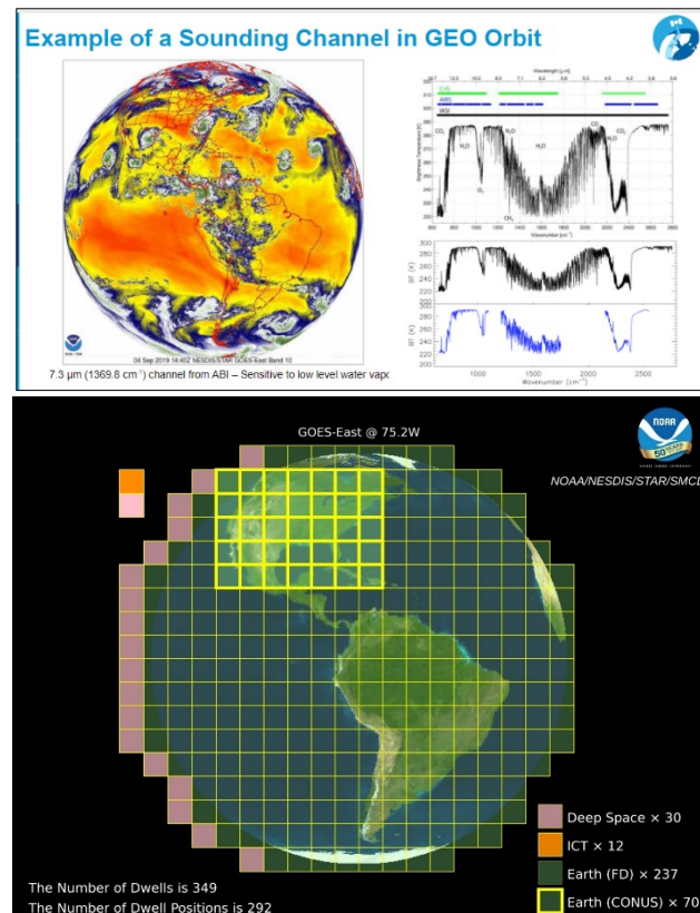
Figure 23. Top: an example of a simulated sounding channel in GEO from the ABI 7.3\mu\text{m} ( 1369.8\text{ cm}^{-1} ) channel – sensitive to low-level water vapor. Bottom: a proposed GEO hyperspectral IR sounder 60-min scanning scheme designed to cover the CONUS every 30 minutes and the full disk every 60 minutes.
